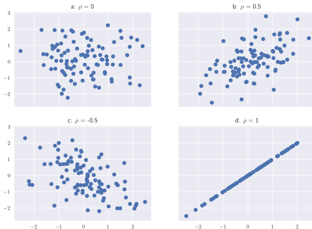
Bivariate Normals
